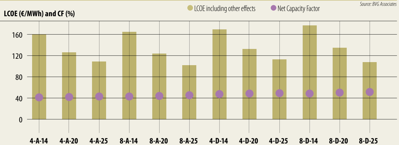
Figure 10.5 LCOE for wind farms with FID 2014, 2020 and 2025 with other effects incorporated, ref. Section 2.4.
