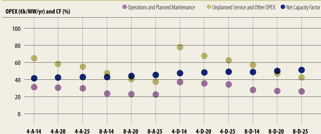
Figure 10.4 OPEX and net capacity factor for wind farms with FID 2014, 2020 and 2025.
